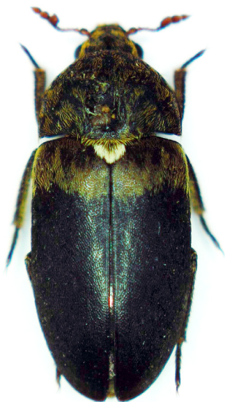
Figs. 3-4. Dermestes (Dermestinus) solskyi Dalla Torre, 1911: 3- habitus, dorsal aspect; 4- known locality in Iran (asterisk - holotype).
